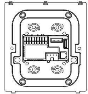
4 BACK VIEW
